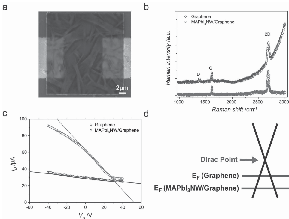
Figure 1. a) Combined optical and SEM image of a representative device showing a random percolating network of MAPbI 3 NWs. b) Raman spectra of the graphene before (paler line) and after (darker line) the deposition of the MAPbI 3 nanowires (spectra are vertically shifted for clarity). c) Transfer characteristic of a representative device without illumination, before (paler line) and after (darker line) the deposition of the network of MAPbI 3 nanowires. d) Dirac cone scheme of the graphene before (paler line) and after (darker line) the hybridization. Note, that the pristine graphene FETs did not show measurable photocurrent under the illumination with 633 nm and 42.5 nW mm -2 .
